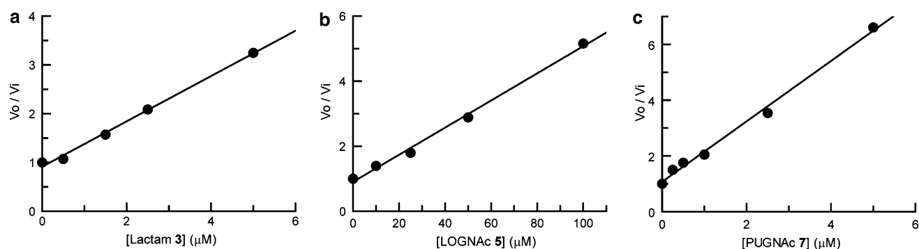
Fig. 2 Plot of v_0/v_i against inhibitor concentration for a 3 , b 5 and c 7 with BtGH84 . Reaction rate is determined by measuring the release of 4-nitrophenolate in the absence ( v_0 ) and presence ( v_i ) of inhibitor. The 1/K_i values for each compound were derived from the slope of the best fit line. Assays were carried out in 50 mM MES, pH 6.5, 200 mM NaCl
