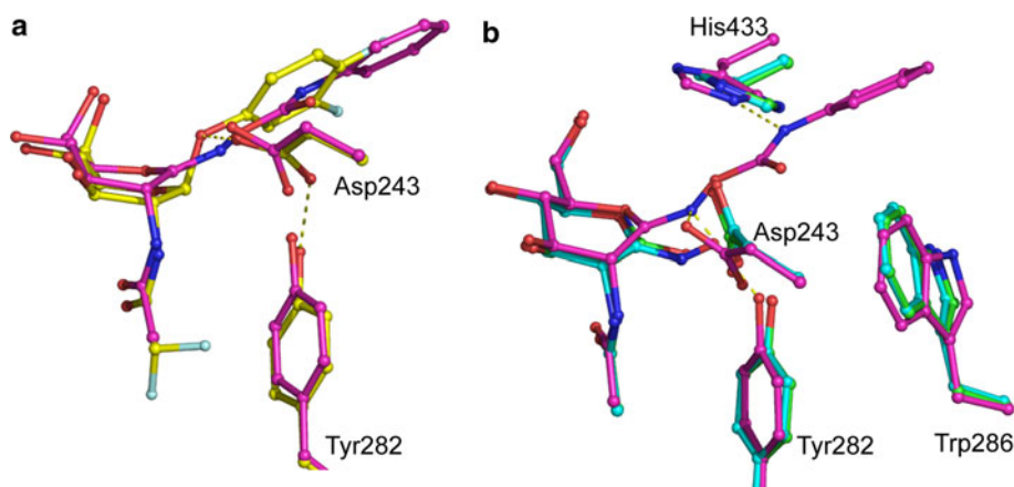
Fig. 5 a Structure of Bt GH84 in complex with PUGNAc (purple) superimposed with the Michaelis complex (yellow). The aglycone moiety of PUGNAc resembles the leaving group in the Michaelis complex in terms of conformation ( {}^{1,4}B ) and the pseudo-axial position of the group in the +1 subsite, which allows a hydrogen bond interaction (represented by a dashed line) between the catalytic acid (Asp243) and the glycosidic oxygen atom in the Michaelis complex. b Superimposition of Bt GH84 in complex with PUGNAc ( 7 ) (purple),
